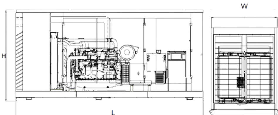
Generator with Soundproof and Containerize Canopy
