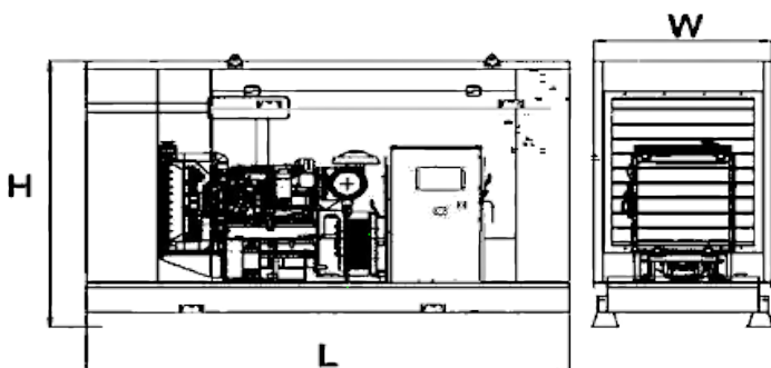
Generator with Soundproof and Round Canopy
