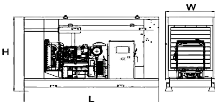
Generator with Soundproof and Round Canopy
